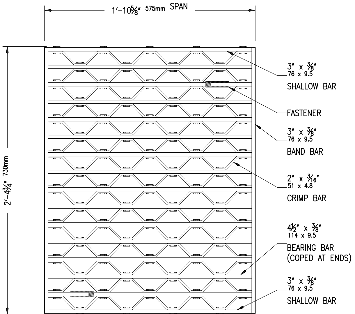
PLAN VIEW SCALE: 2"=1'-0"
