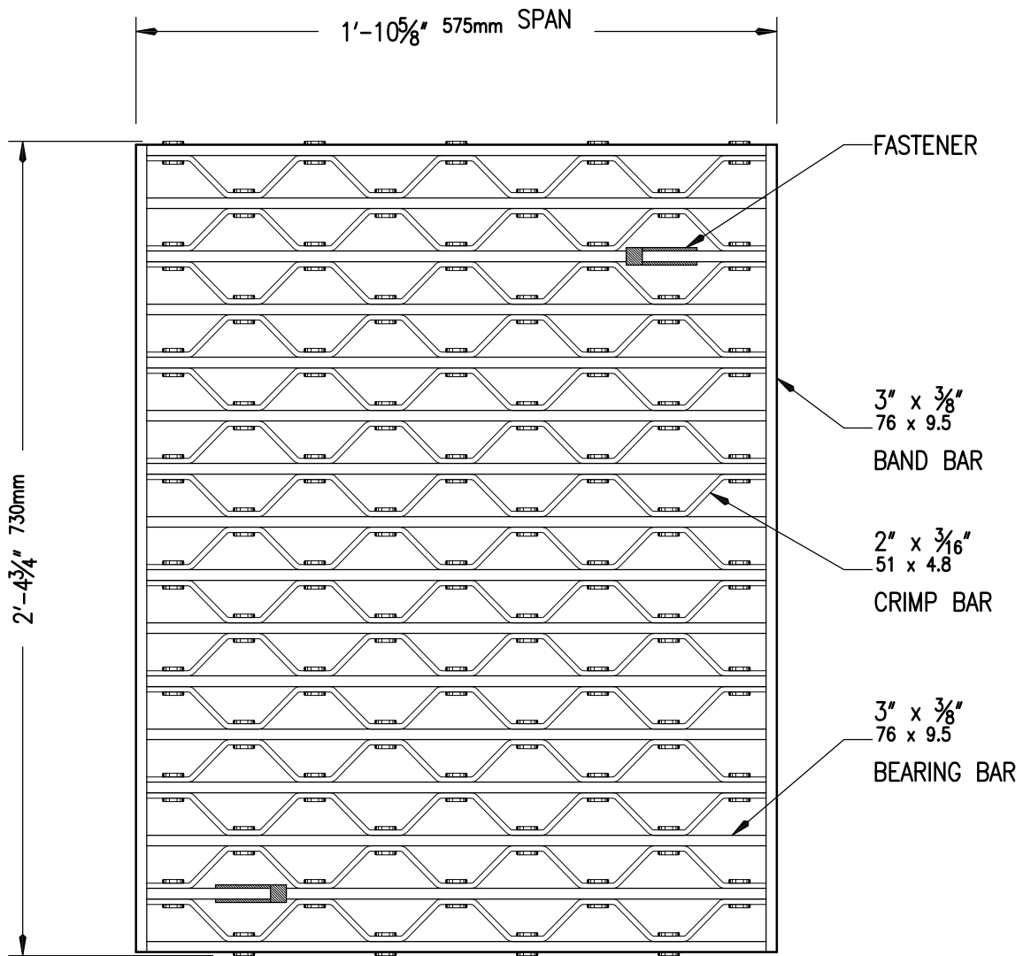
PLAN VIEW SCALE: 2"=1'-0"
